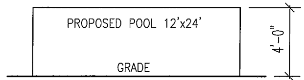
POOL ELEVATION
